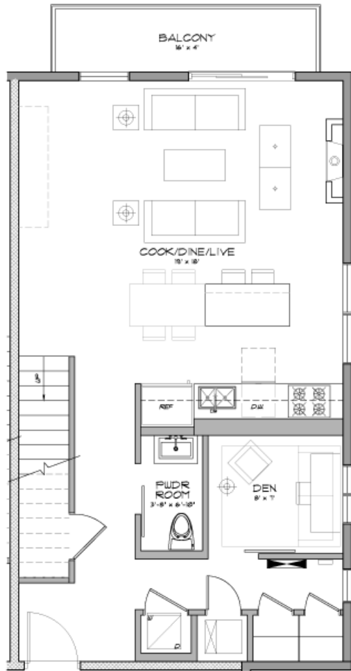
UNIT TYPE A2 -1,350 S.F.
